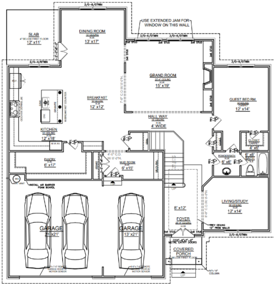
VENUS FIRST FLOOR PLAN ROCKWATER LOT 10
